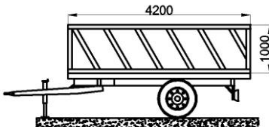
Agro 65 BT 4,2x2,2x1,0m
